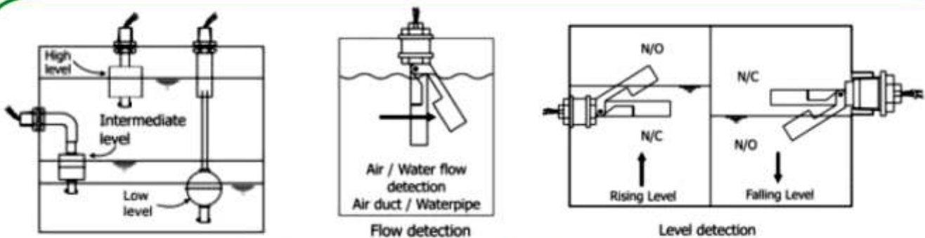
Installation of Top Mounted and Side Mounted Mini Level Switch
