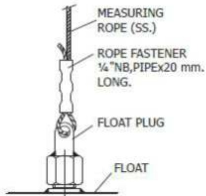
FLOAT ASSEMBLY
