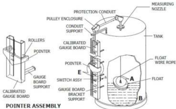
FLOAT & BOARD LEVEL INDICATOR ASSEMBLY WITHOUT GUIDE WIRES
