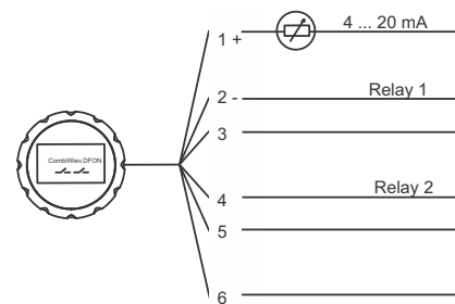
Rear connection
