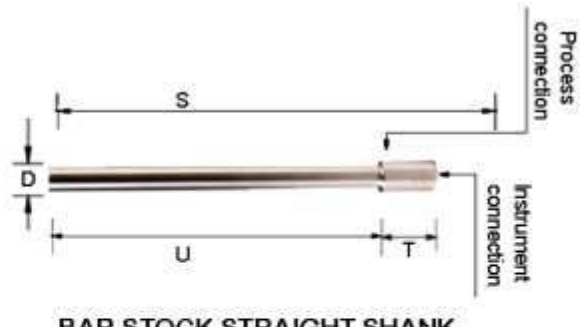
BAR STOCK STRAIGHT SHANK SOCKET WELD THERMOWELL
