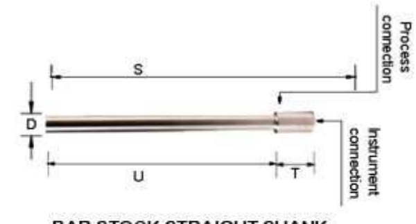
BAR STOCK STRAIGHT SHANK SOCKET WELD THERMOWELL
