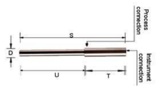
WELDED STRAIGHT SHANK WITH LAG SOCKET WELD THERMOWELL
