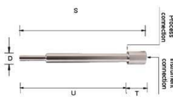
WELDED REDUCED TIP SOCKET WELD THERMOWELL
