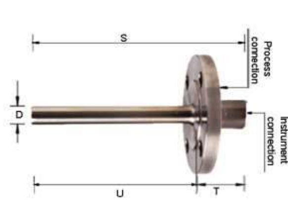
WELDED STANDARD FLANGE THERMOWELL
